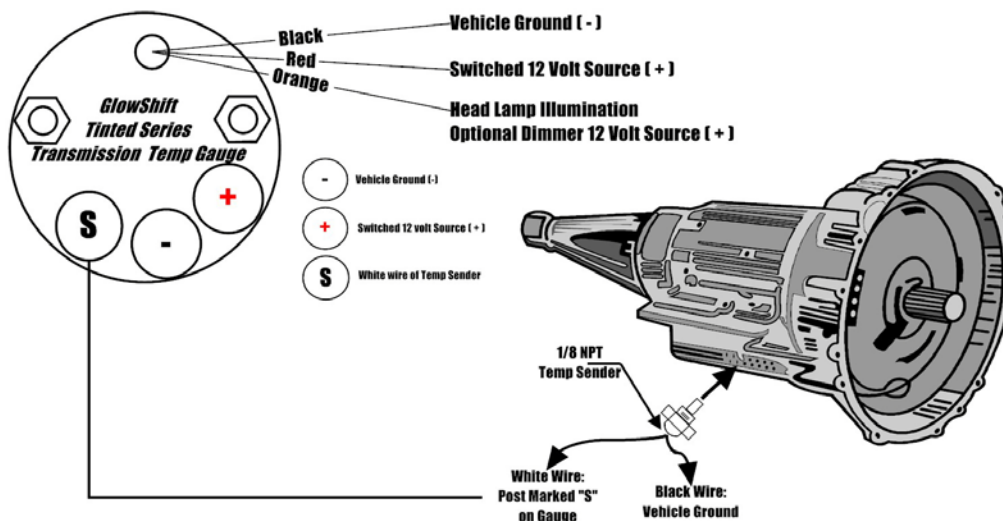
Wire Color Code
