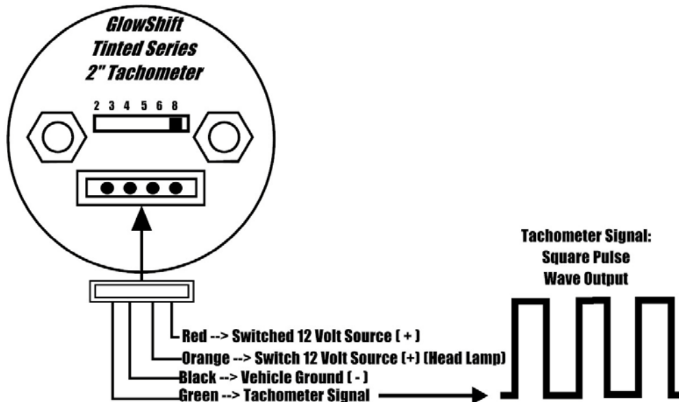
Wire Color Code
