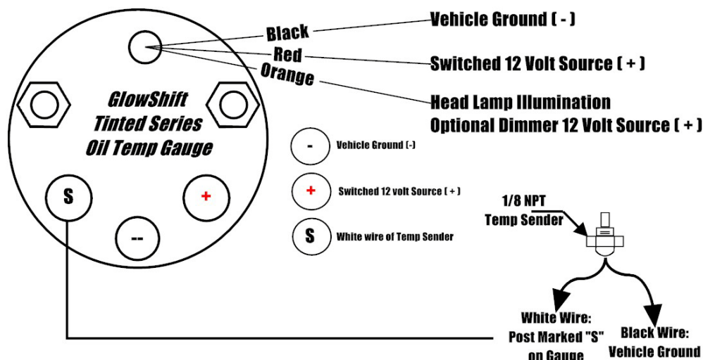
Wire Color Code
