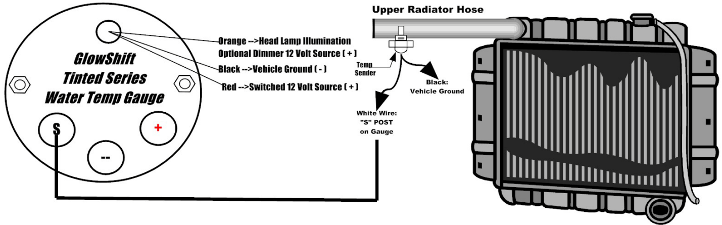
Wire Color Code
