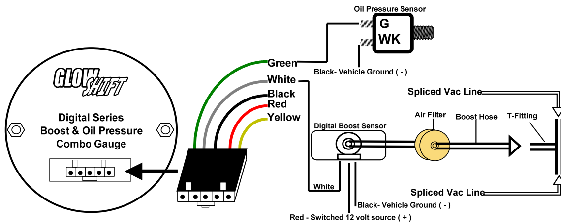
Wire Color Code
