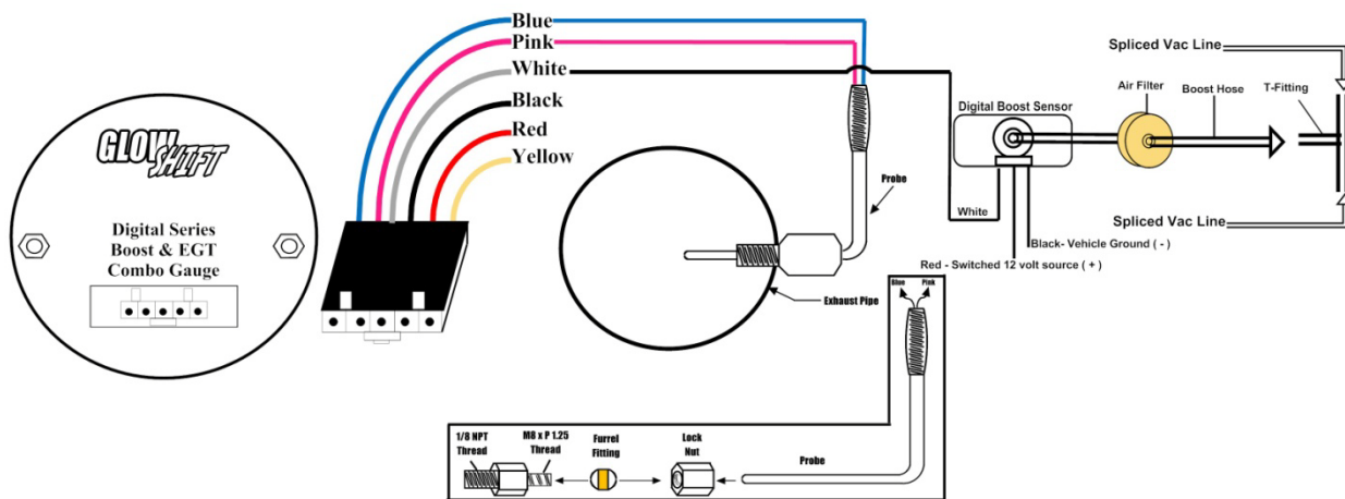
Wire Color Code
