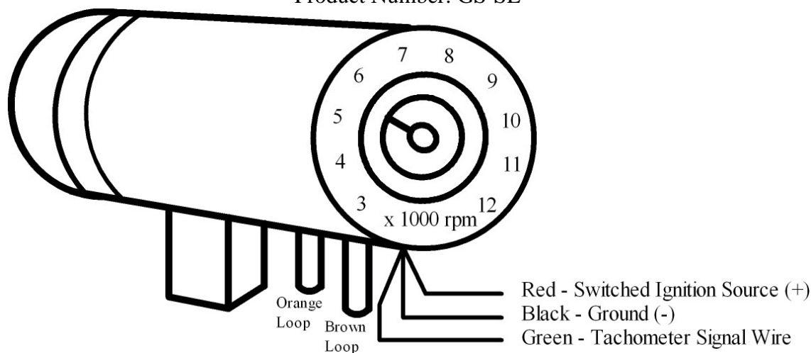
Wire Color Code
