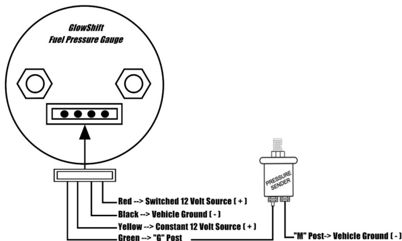
Wire Color Code
